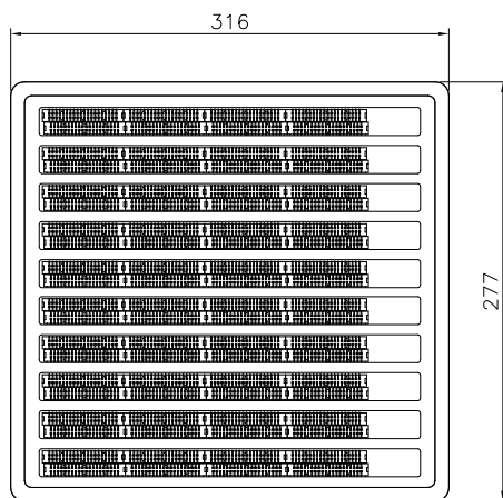
TRAY LAYOUT
